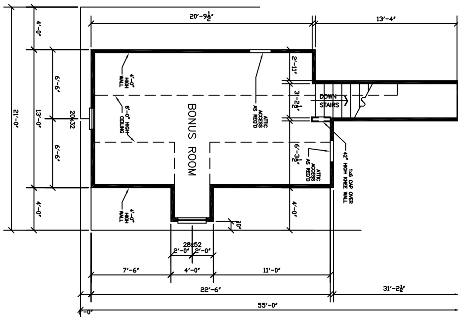
BONUS ROOM PLAN SCALE: 1/4-IN. = 1'-0"
